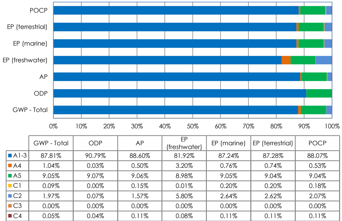
Figure 1 - shows the relative contribution of each life cycle stage to different environmental indicators for the carbon steel reinforcing bar products manufactured by the primary (BF-BOF), DRI and the secondary (scrap-based) production routes
